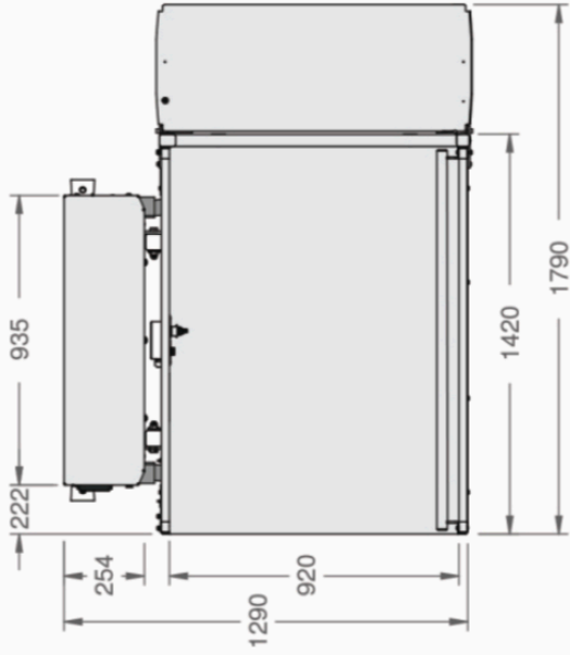
PLAN ELEVATION THROUGH PLATFORM
